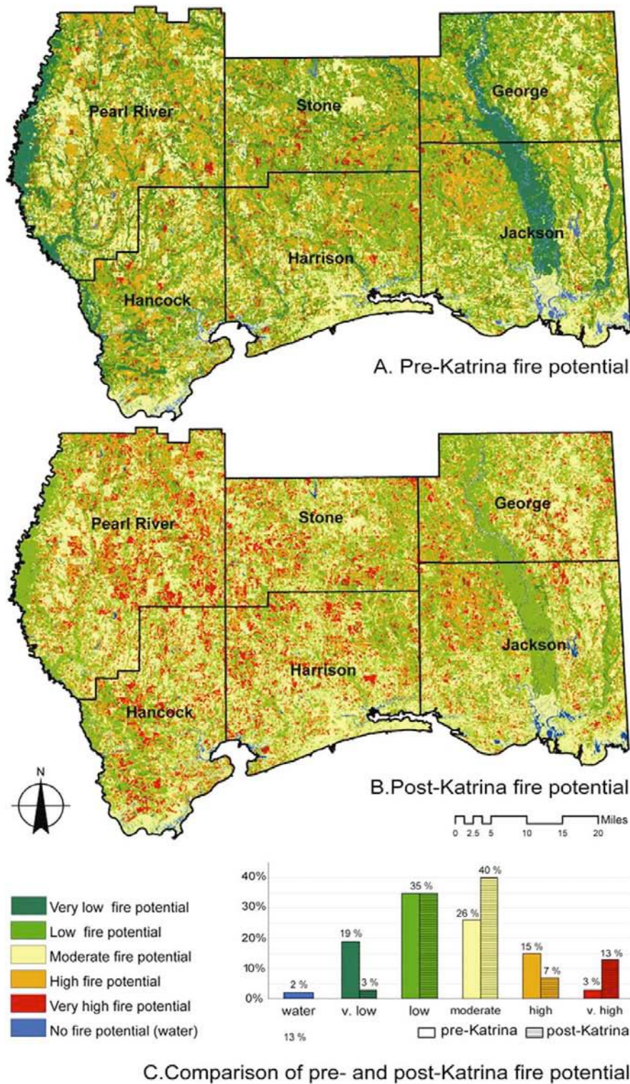
Figure 7 — Pre- and post-Katrina fire potential comparison for six southern Mississippi counties.
